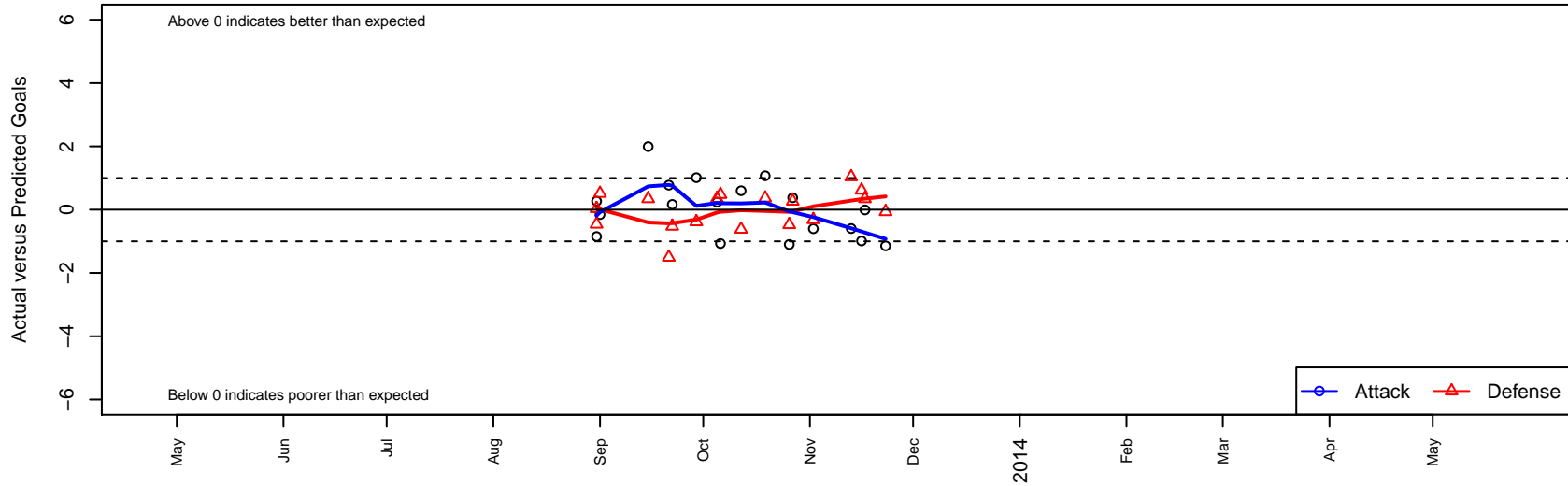
Laguna Hills Eclipse White G00 Dots are actual minus expected GF (blue circles) and GA (red triangles). Blue line is smoothed change in attack strength. Red is smoothed change in defense strength.
